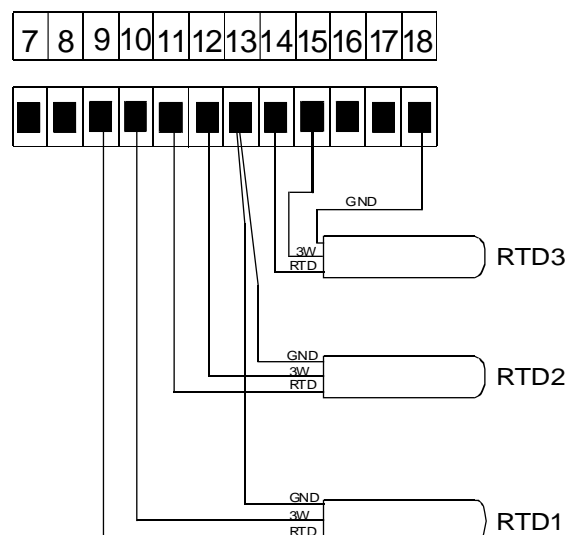
Example - 3 x 3 wire RTD
