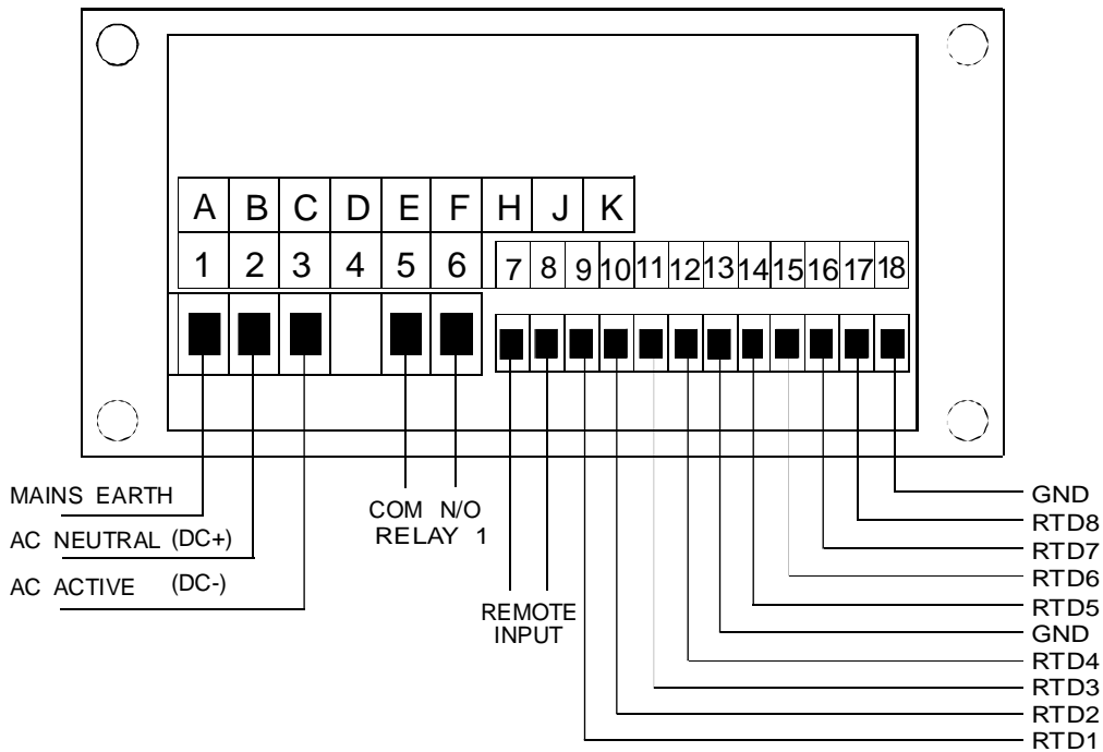
Instrument rear panel - 2 wire connection
